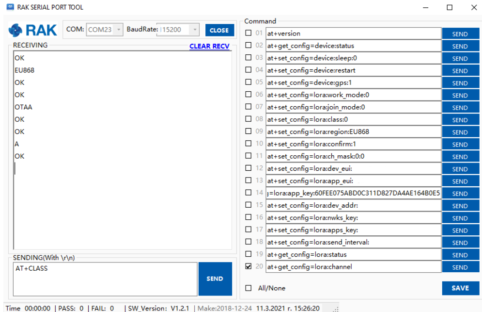
Figure 59: Setting up the RAK7431 WisNode Bridge Serial operation modes
