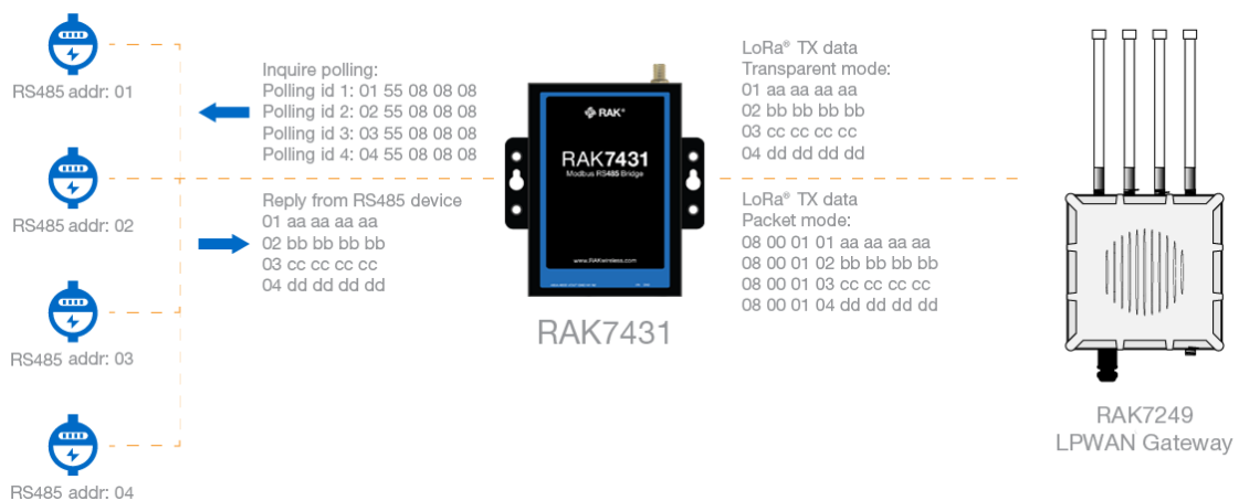
Figure 12: Scheduled polling example
