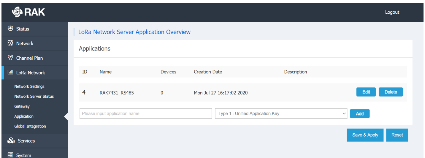
Figure 6: Application list
