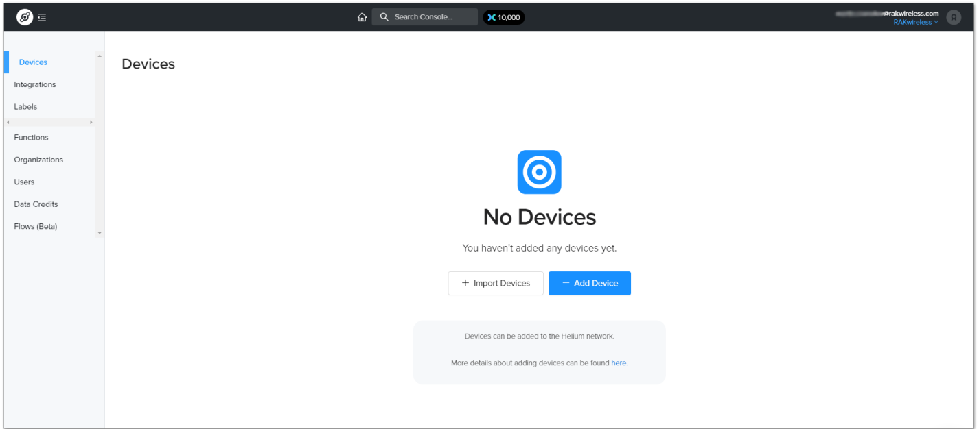
Figure 45: Devices Section
