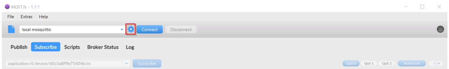
Figure 16: MQTT.fx Client
