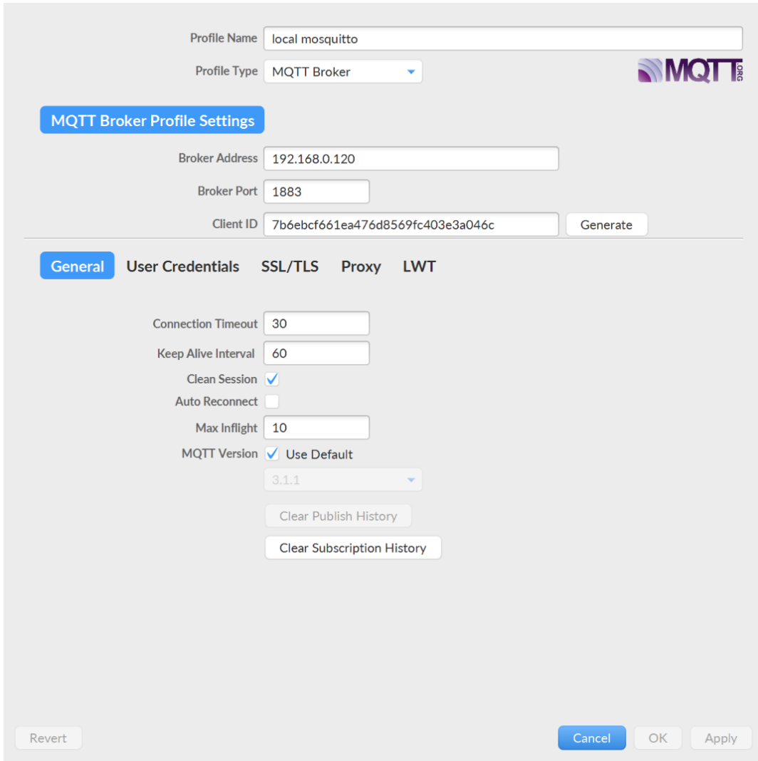
Figure 17: MQTT.fx settings
